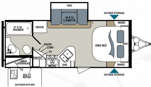
AEROLITE LUXURY CLASS | 213RBSL Ext. Length: 25' 8" Ext. Height: 11' 1" Average Shipping Weight: 4,973 Sleeps: 4
