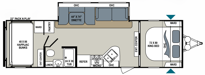
AEROLITE LUXURY CLASS | 292DBHS Ext. Length: 34' Ext. Height: 11' 1" Average Shipping Weight: 6,452 Sleeps: 10
