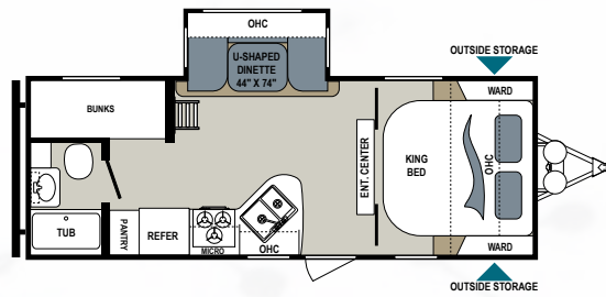
AEROLITE LUXURY CLASS | 221BHSL Ext. Length: 26' 7" Ext. Height: 10' 10" Average Shipping Weight: 5,230 Sleeps: 6
