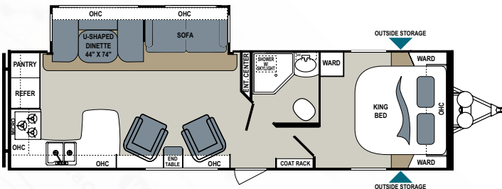
AEROLITE LUXURY CLASS | 294RKSS Ext. Length: 34' 2" Ext. Height: 11' Average Shipping Weight: 6,359 Sleeps: 6
