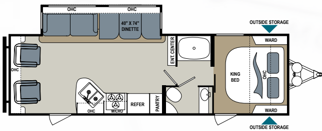
AEROLITE LUXURY CLASS | 281RLSS Ext. Length: 32' 2" Ext. Height: 11' 2" Average Shipping Weight: 6,246 Sleeps: 6
