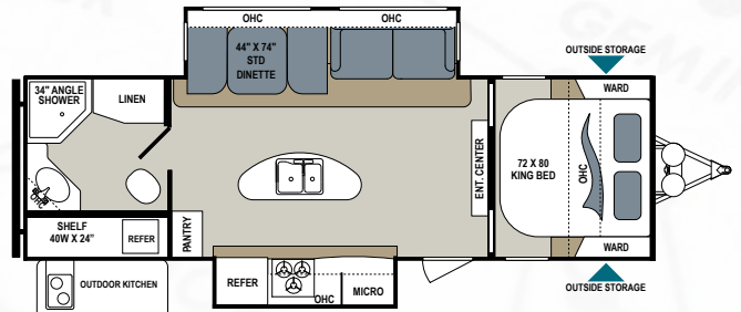
AEROLITE LUXURY CLASS | 272RBS5 Ext. Length: 31' 9" Ext. Height: 11' 1" Average Shipping Weight: 6,600 Sleeps: 6
